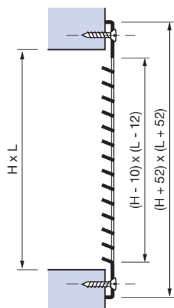
type GK 150 Fixing with visible screws
